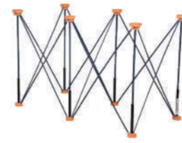
71926 2ft x 4ft, 36" Work Height 2,500 lbs Loading Capacity
