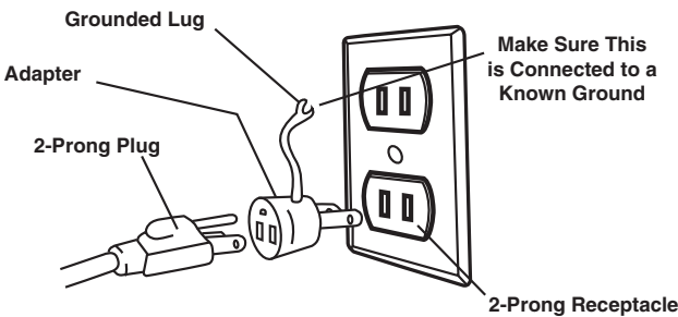
Figure 6 - 2-Prong Receptacle
