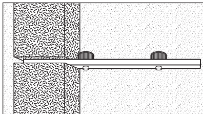
Gauge standard brick joints (10 mm)
