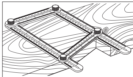
Make a template to cut birds mouth rafters
