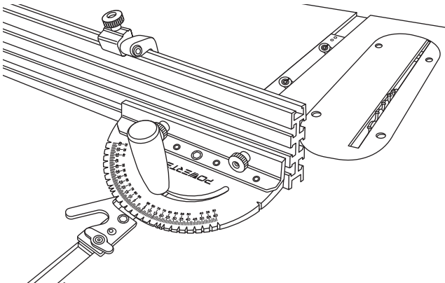
Use with the 71142, Powertec V27 Miter Gauge
