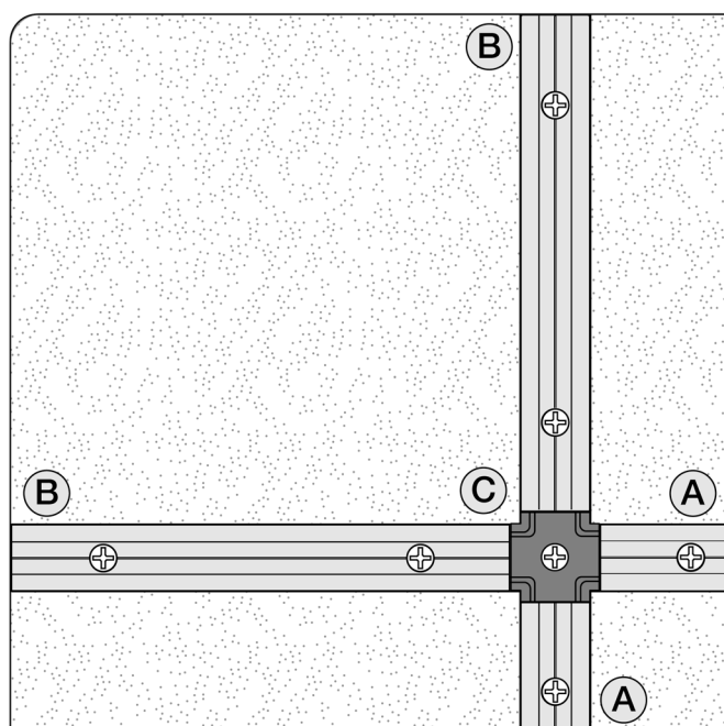
Figure 5 Place 4-Way Drop-In Intersections (C) and secure with wood screws.
