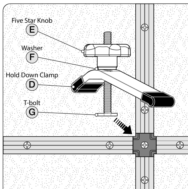
Figure 6 Insert T-bolt of Hold Down Clamp into any of the 8 intersections, position as needed.
