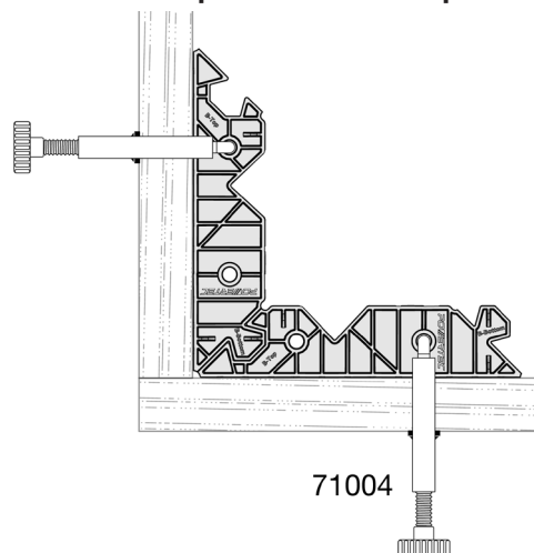
Figure 9 Example of Inside Setup
