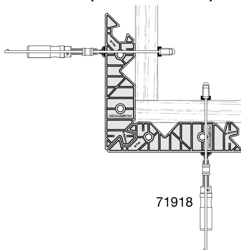
Figure 10 Example of Outside Setup
