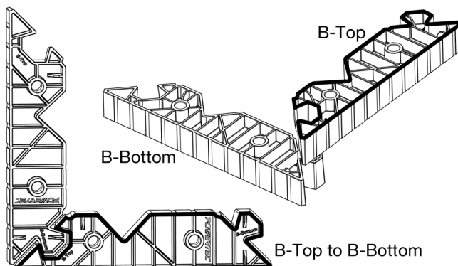
Figure 9 Example of Inside Setup
