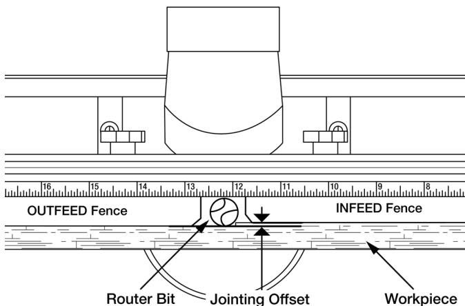
Figure 17-b (Top View with workpiece)
